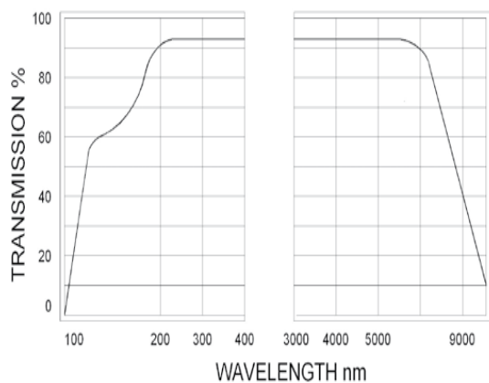
Magnesium fluoride transmission curve
