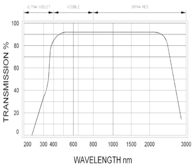
Kodial transmission curve
