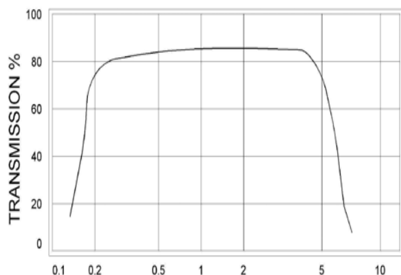
Sapphire zero length transmission curve
